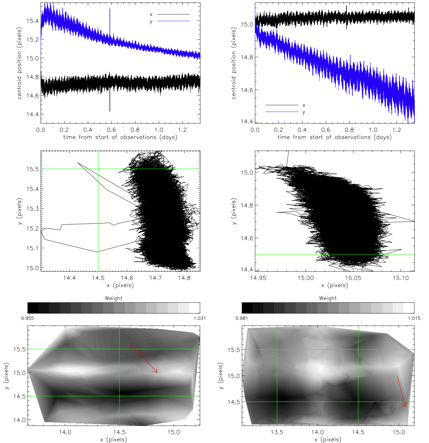
Figure 2. Point-spread function centroid movement at 3.6\ \mu\text{m} (left) and 4.5\ \mu\text{m} (right). The top panels show the jitter and drift of the PSF centroid. The second panels show the two-dimensional wander of the centroid. The bottom panels show the intra-pixel sensitivity map for the central regions of the detector, constructed by applying the Ballard et al. (2010) point-by-point decorrelation to our mapping data (see Section 3.2.2), with red arrows marking the approximate drift of the PSF over the course of our observations. The green lines show pixel edges.
